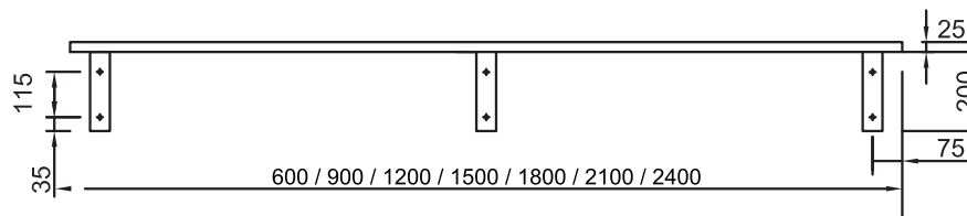
FRONT ELEVATION
